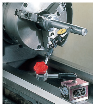
On NC Lathe
